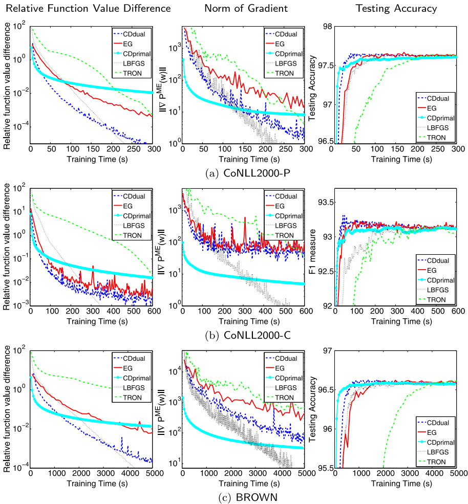
Fig. 3 Results for maximum entropy on 0/1-feathered data. The first column shows time versus the relative function difference (55). The second and third columns show \|\nabla P^{ME}(\mathbf{w})\| and testing performances along time, respectively. Time is in seconds
