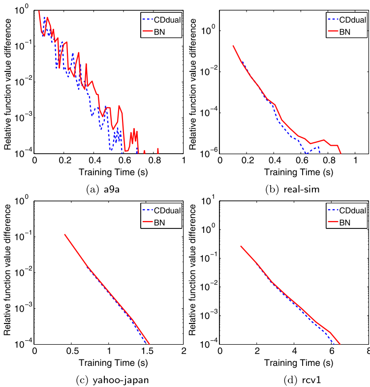
Fig. 4 A comparison between BN and CDdual on logistic regression for real-valued document data. The figures show time versus the relative function value difference defined in (55). Time is in seconds
