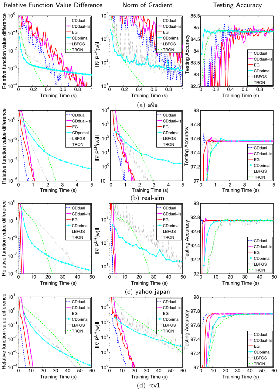
Fig. 2 Results for logistic regression on real-valued document data. The first column shows time versus the relative function difference (55). The second and third columns show \|\nabla P^{LR}(\mathbf{w})\| and testing performances along time, respectively. Time is in seconds
