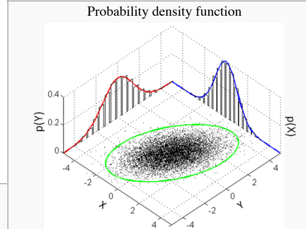
Many samples from a multivariate normal distribution, show along with the 3-sigma ellipse, the two marginal distribution and the two 1-d histograms.
