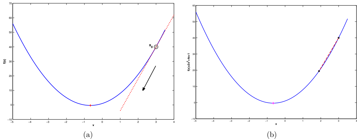
Figure 3: (a) A plot of the function f(x) = 3x^2 + 4x + 1 and the tangent to the function at x_0 = 3 , if we move in the direction as shown we will be getting closer to the function minimum. (b) shows the next point x_1 that we reach by moving in the shown direction, which is closer to the minimum.
