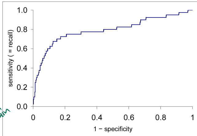
Figure 2: ROC Curve
