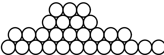
Fig. 2.1: A (28, 12) fountain
