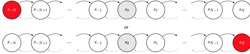
Figure 19: MDPs where Thompson sampling every timestep leads to inefficient exploration.
