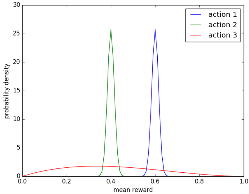
Figure 3: Probability density functions over mean rewards.
