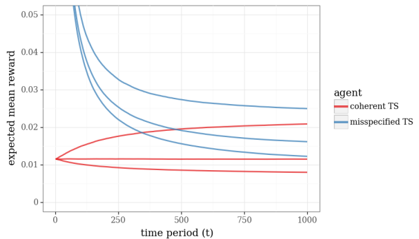
(b) expected mean rewards
