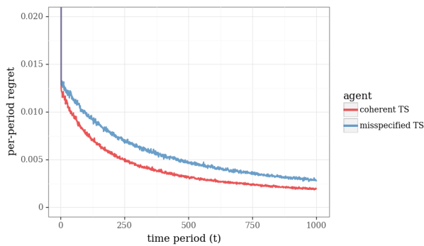
(a) regret
