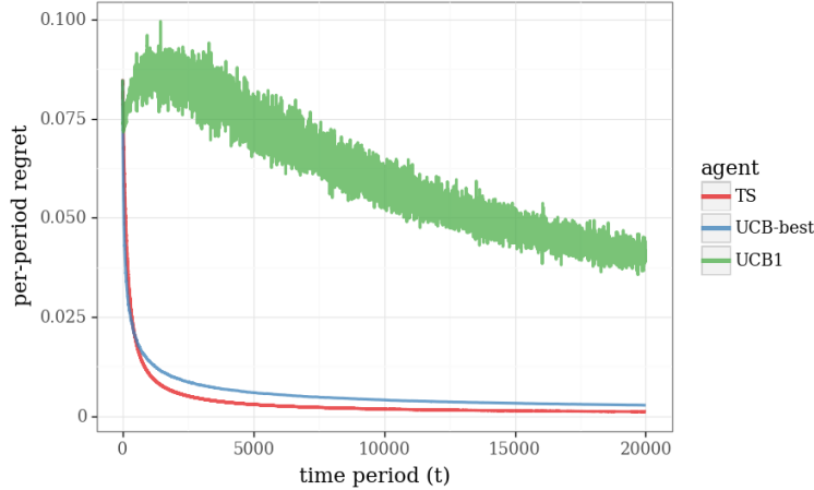
Figure 15: Comparison of CascadeTS and CascadeUCB with K = 1000 items and J = 100 recommendations per period.
