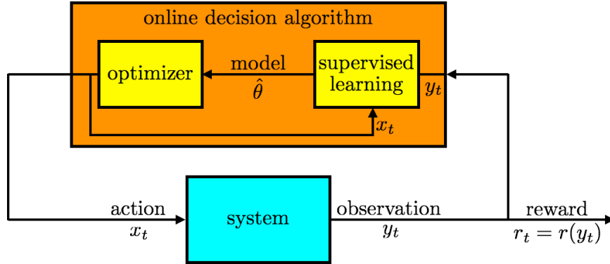
Figure 2: Online decision algorithm.
