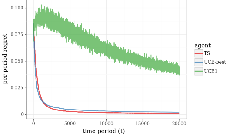
Figure 17: Comparison of CascadeTS and CascadeUCB, both initialized with uniform priors, with K = 1000 items and J = 100 recommendations per period.
