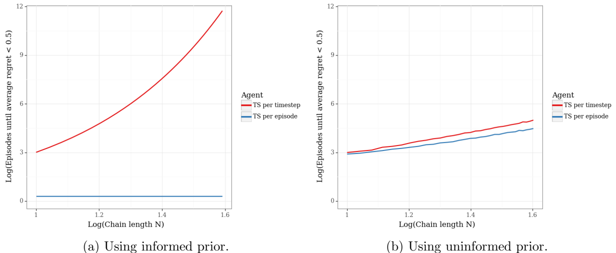
Figure 20: Comparing Thompson sampling by episode with Thompson sampling by timestep.
