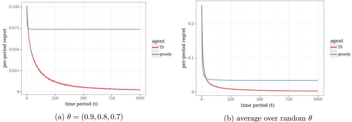
Figure 5: Regret from applying greedy and Thompson sampling algorithms to the three-armed Bernoulli bandit.
