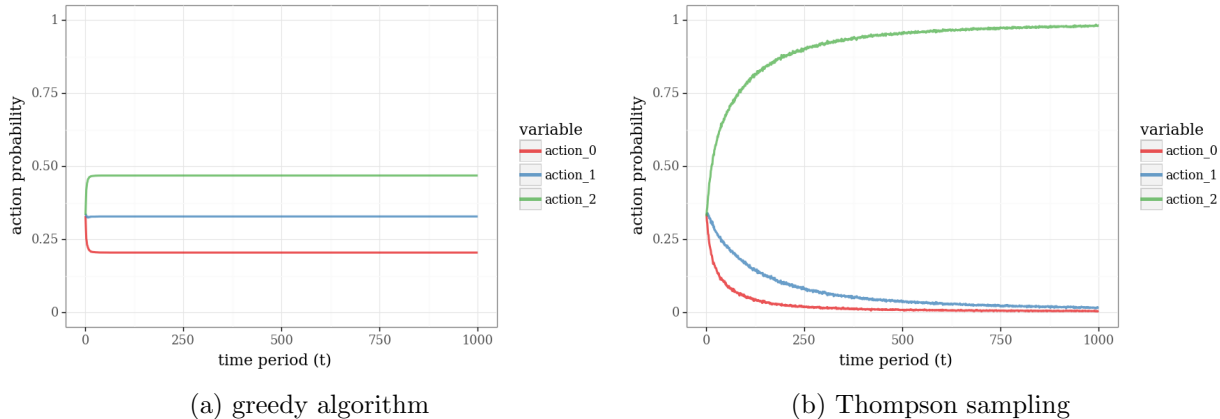
Figure 4: Probability that the greedy algorithm and Thompson sampling selects an action.
