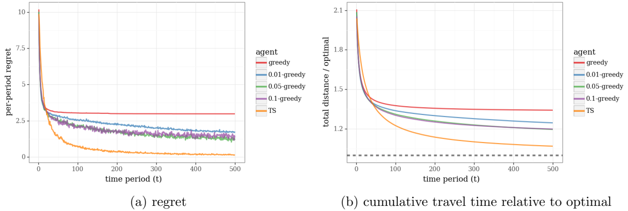
Figure 7: Performance of Thompson sampling and \epsilon -greedy algorithms in the shortest path problem.
