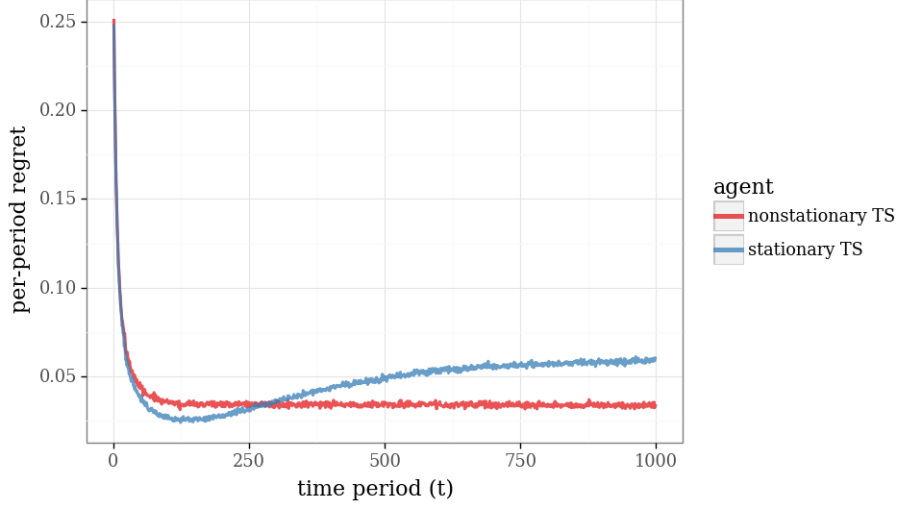
Figure 13: Comparison of Thompson sampling versus nonstationary Thompson sampling with a nonstationary Bernoulli bandit problem.
