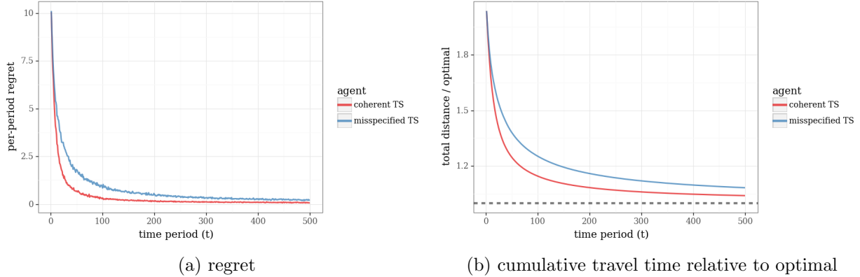
Figure 8: Performance of two versions of Thompson sampling in the shortest path problem with correlated travel times.
