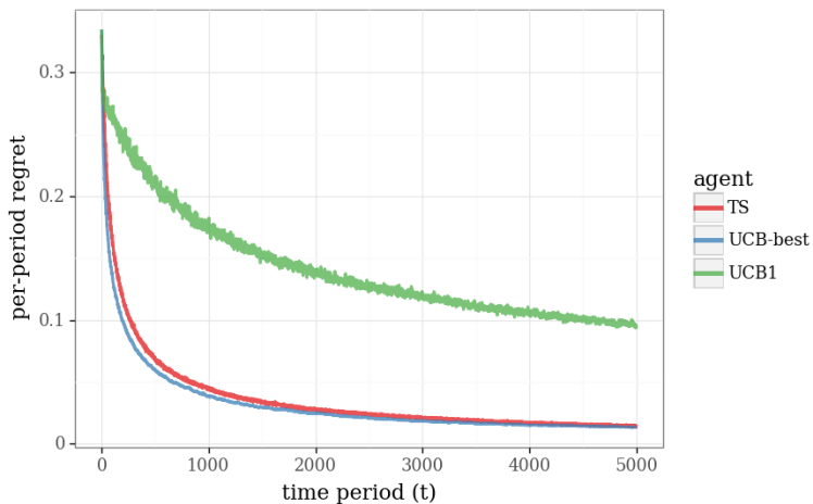
Figure 16: Comparison of CascadeTS and CascadeUCB with K = 50 items and J = 10 recommendations per period.
