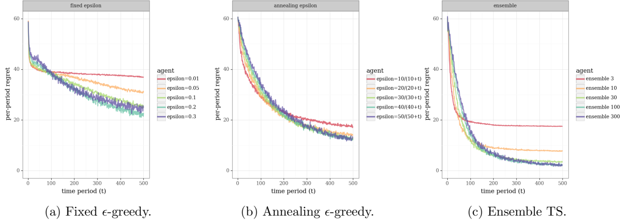
Figure 18: Bandit learning with an underlying neural network.
