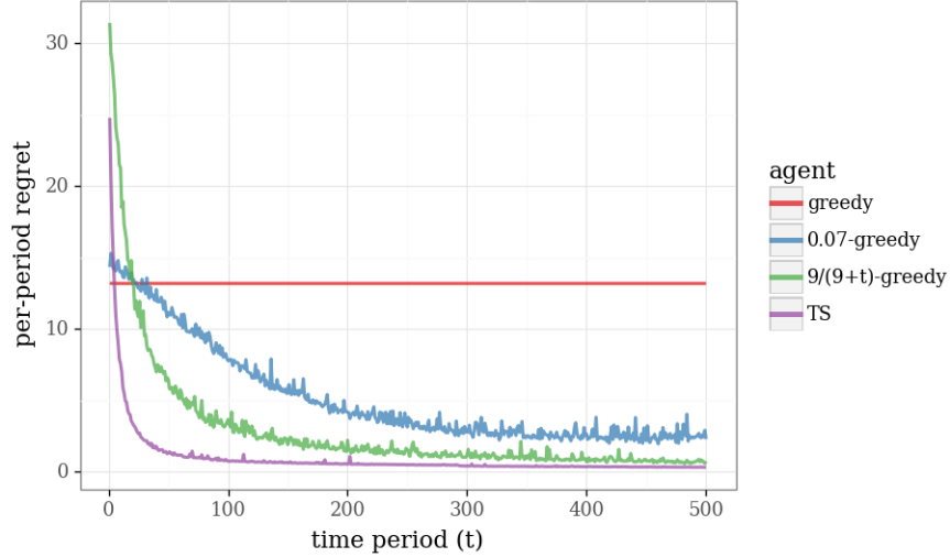
Figure 14: Regret experienced by different learning algorithms applied to product assortment problem.
