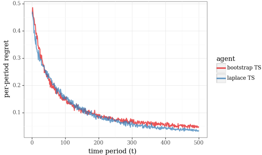
Figure 9: Regret experienced by approximation methods applied to the path recommendation problem with binary feedback.
