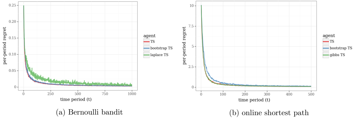
Figure 10: Regret of approximation methods versus exact Thompson sampling.
