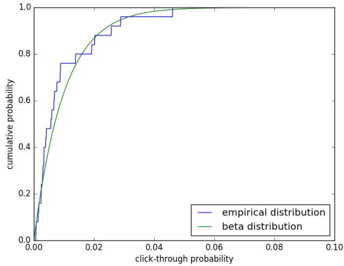
Figure 11: An empirical cumulative distribution and an approximating beta distribution.
