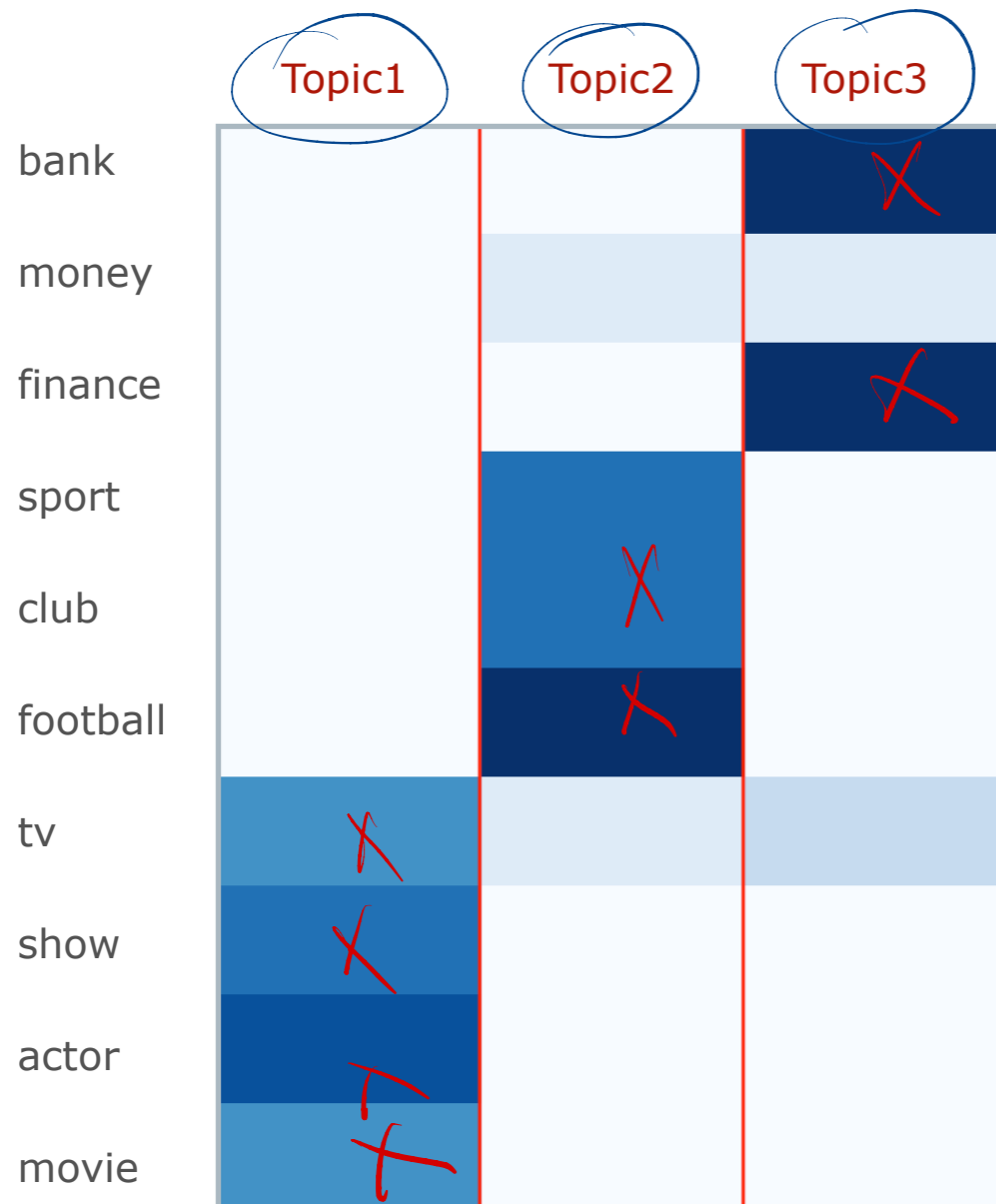
Basis vectors W : topics (clusters)
