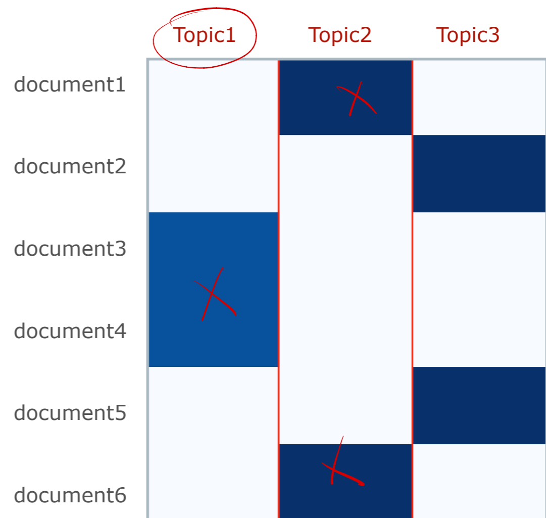
Coefficients H : memberships for documents
