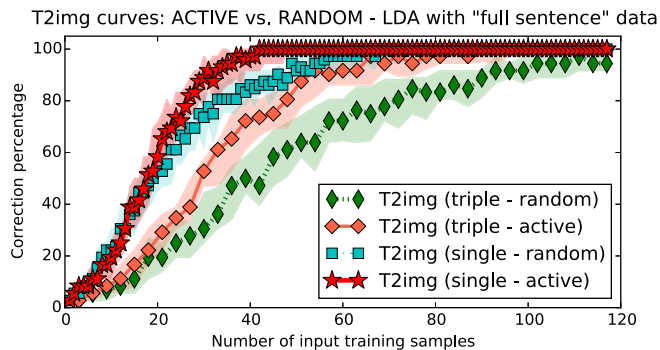
Fig. 6. Comparison between active learning and random learning by applying NMF (left) or LDA (right) with “full sentence” data
