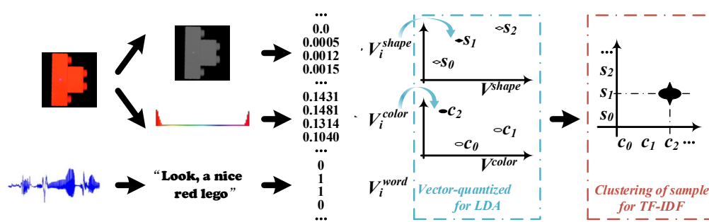
Fig. 2. Illustration of the data representation used in our experiments.
