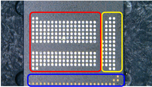
Figure 5: Pin layout of Hynix BGA221 eMMC ICs, with DDR RAM (red), eMMC (yellow) and NAND test pads (blue)
