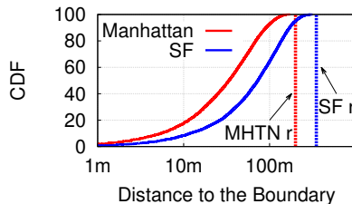
Figure 6: Distance of short-lived insiders to the boundary.
