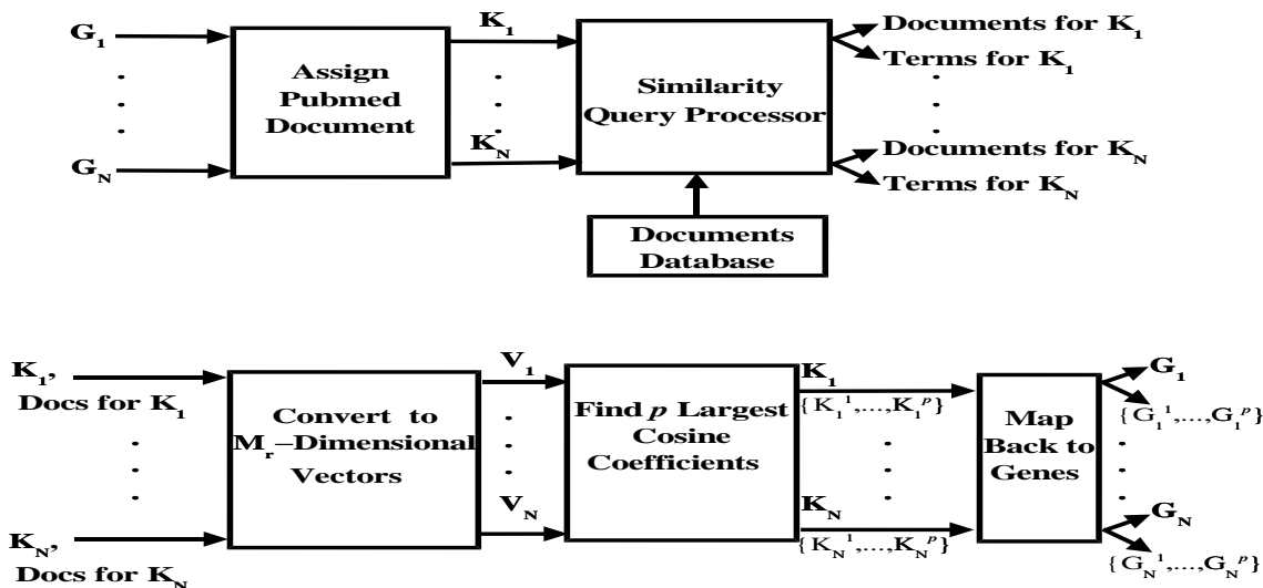
Figure 7: Finding documents and terms related to genes (top), and sets of related genes (bottom).
