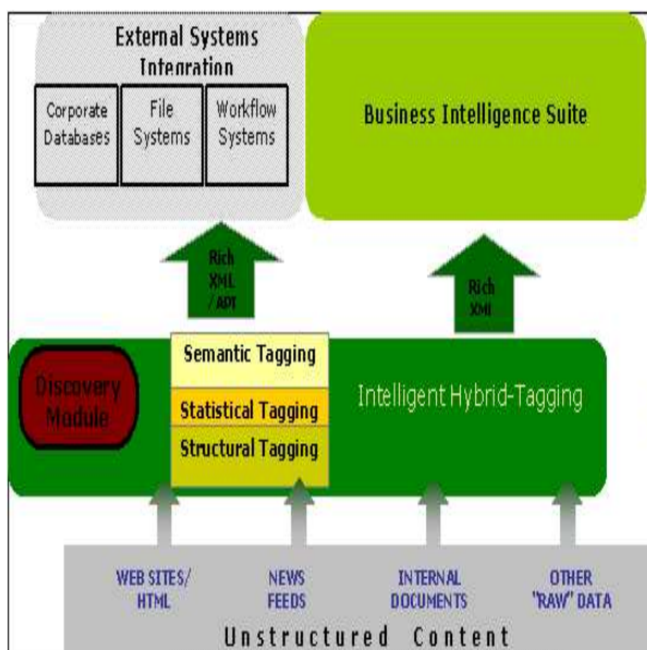
Figure 8: Architecture of the LitMiner system.
