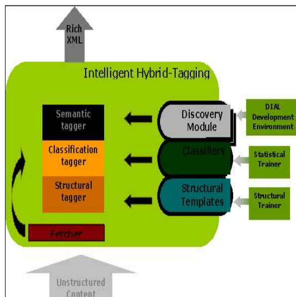
Figure 9: Architecture of the hybrid tagging system.
