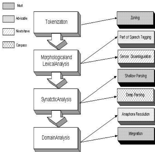
Figure 5: Architecture of a typical Information Extraction system.
