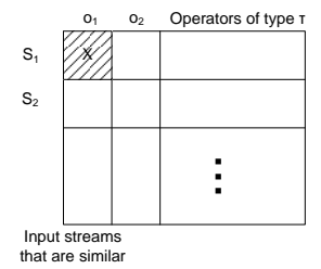
Figure 3: \mathcal{R}_2 Applied to a Set of Operators of Type \tau
